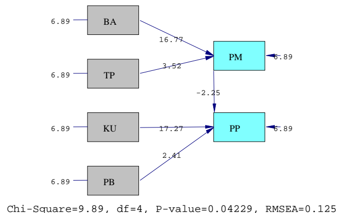
Figure 4: t-Test Path Diagram after Trimming
