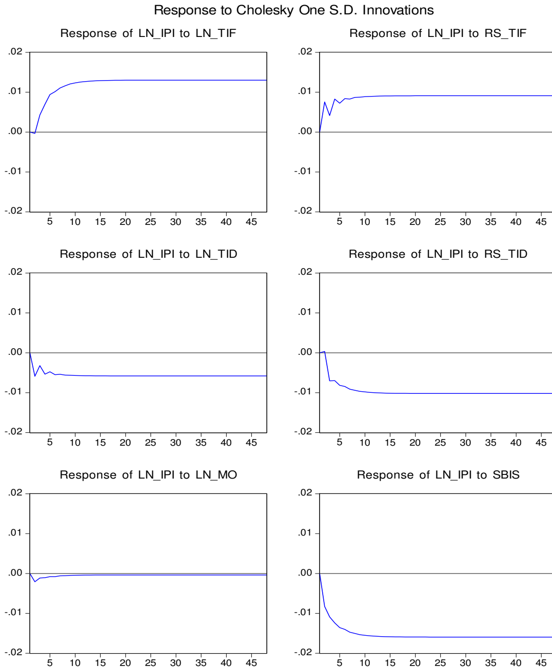
Figure 1. Impulse Response on IPI Model
